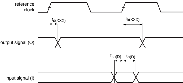
Fig 18. Signal timing
